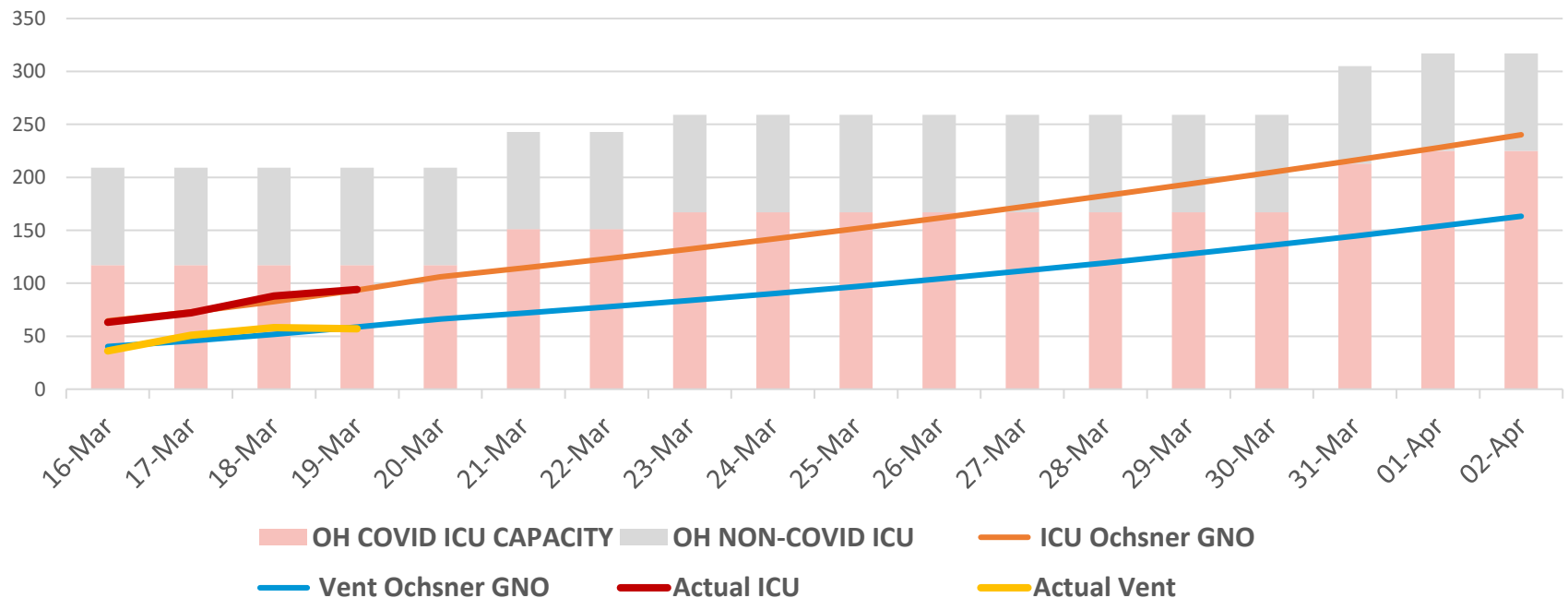
Ochsner GNO 28 Day ICU, Vent Prediction Compared to Actual Social Distancing on 3/16
